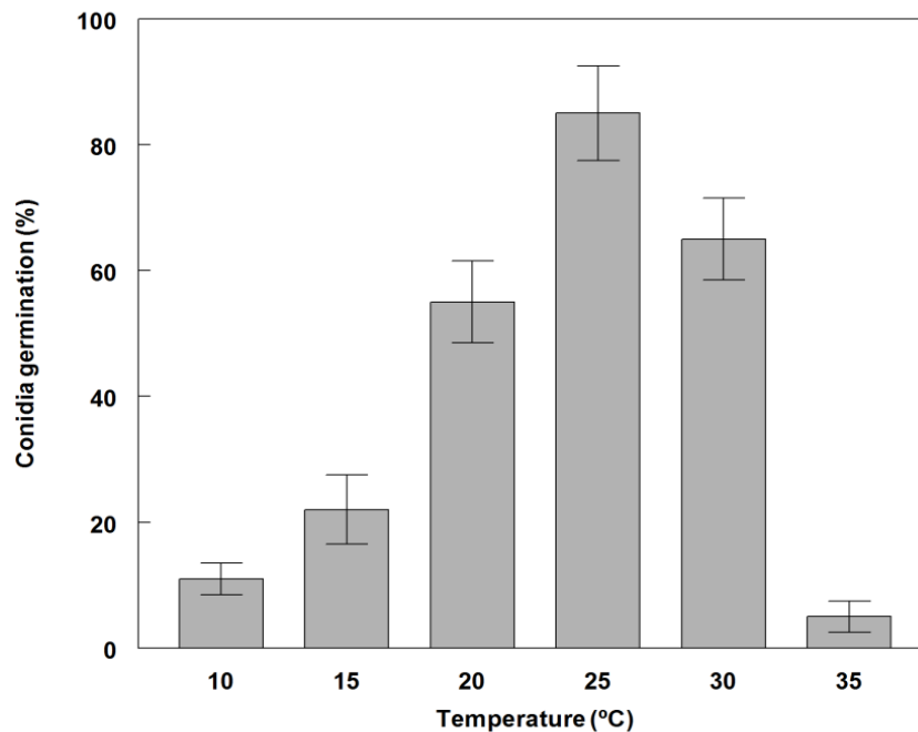
Figure 2. Effect of temperature on germination of conidia of P. commelinicola on PDA, 7 days after inoculation and growth under alternating light/dark conditions (12 h light/dark at 28 °C). Error bars represent Fisher's LSD ( p = 0.05 ).
